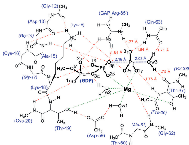
Scheme 1. The QM-derived TS model for GTP hydrolysis by RhoA/GAP showing the H-bonding network for the catalytic region (red dashes) with ligands coordinated to Mg (green dashes). Amino acid residues are numbered according to RhoA sequence plus Arg85' from RhoGAP.
