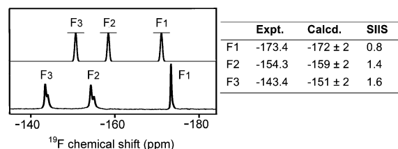
Figure 2. Upper spectrum: Calculated 19 F NMR for the computational model of the RhoA/GAP-GDP-MgF 3 − TSA complex, Lower spectrum: Experimental 19 F NMR of the RhoA/GAP-GDP-MgF 3 − TSA complex. Calculated and experimental 19 F chemical shifts with the measured SIIS are tabulated with fluorines numbered according to corresponding \gamma -oxygens in Scheme 1 (Figure S2).
